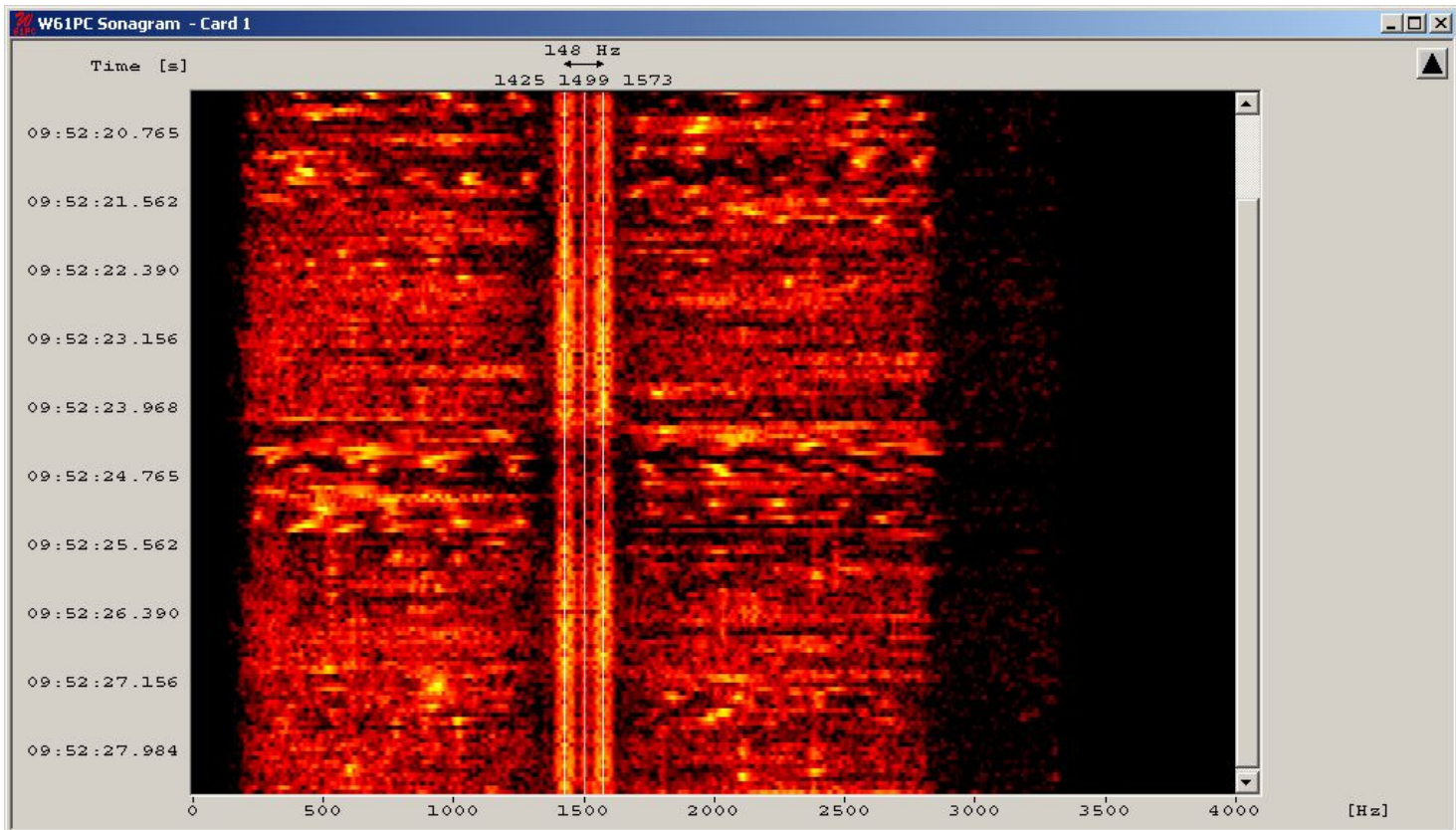
Russian voicescrambler Yakhta inband synchro FSK-signal (100 Bd – 150 Hz shift) on 21001.5 kHz with spurious emissions covering about 8 kHz - Location: Nizhny Tagil - screenshot: DK2OM
